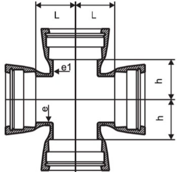
All Socket Cross
