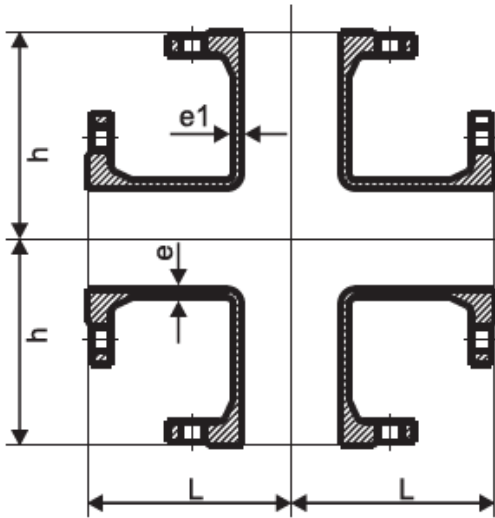
All Flange Cross
